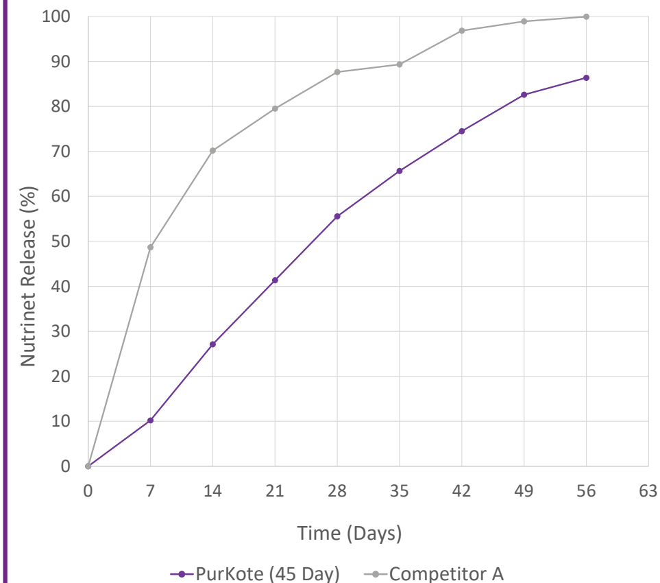
PurKote 45 Day Urea Vs. Competitor 45 Day Urea Dissolution Rate at 87°F (30°C)
